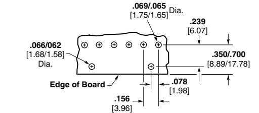
Recommended Mounting Hole Pattern for .062 [1.57] Thick PC Board Using a Right-Angle Header
